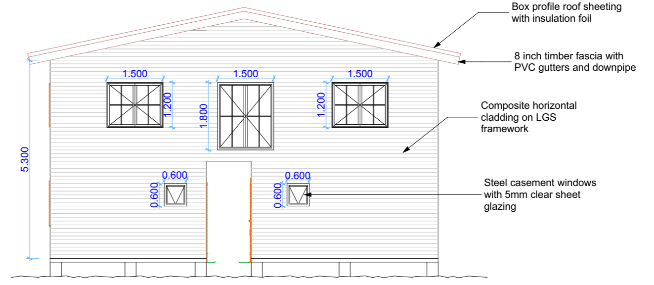
North Elevation
