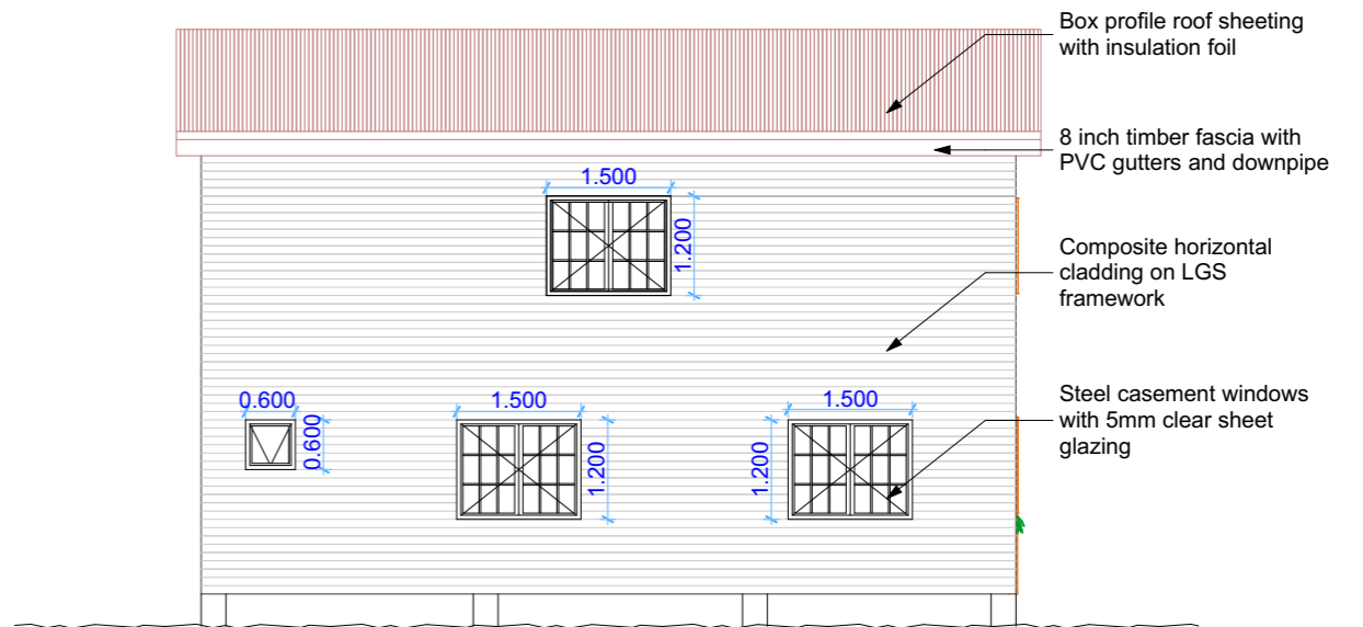
West Elevation
